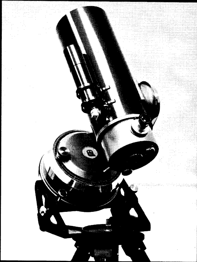
QUANTUM SIX SHOWN ON FOLDING TRIPOD AND WEDGE ASSEMBLY
